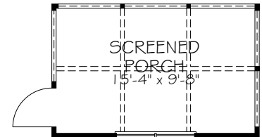
OPTIONAL MASTER SCREENED PORCH 15'-4" x 9'-8"
